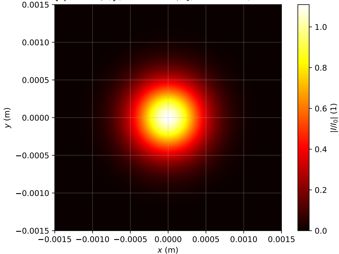
Intensity profile I(x, y, z = 0.478m)/I_0 , P_{in}=0.8P_{cr} , artificial time
